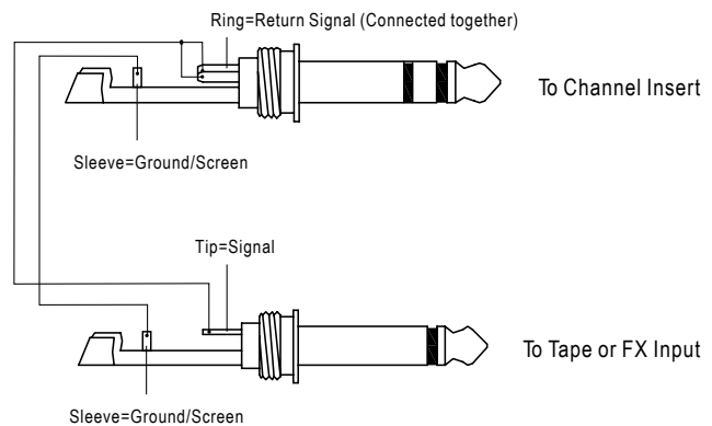
'Tapped' Connection Direct Output Lead
