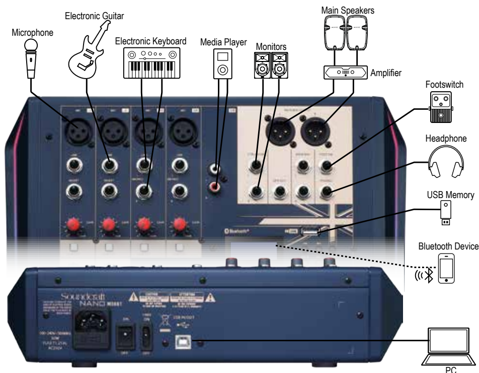
Connection Example
